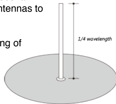
Whip Antenna
